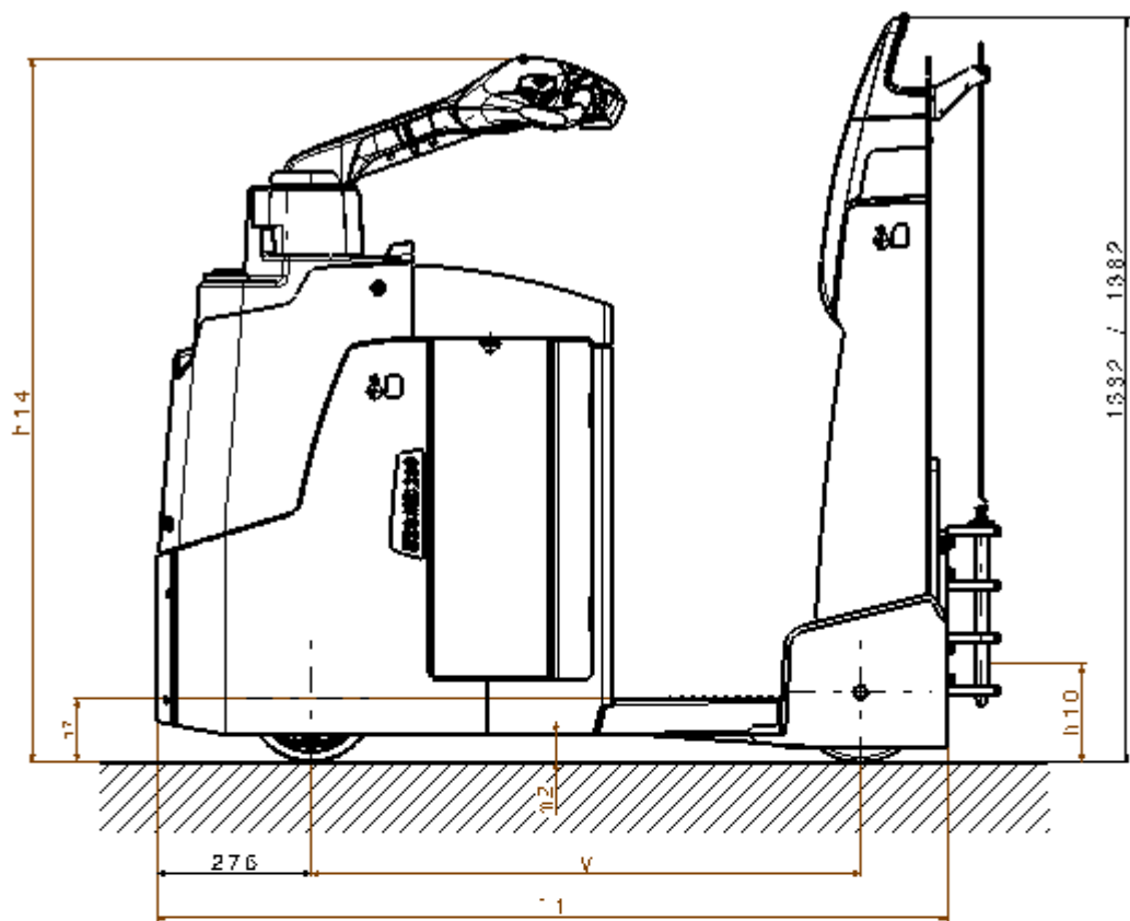
Truck-Layout
